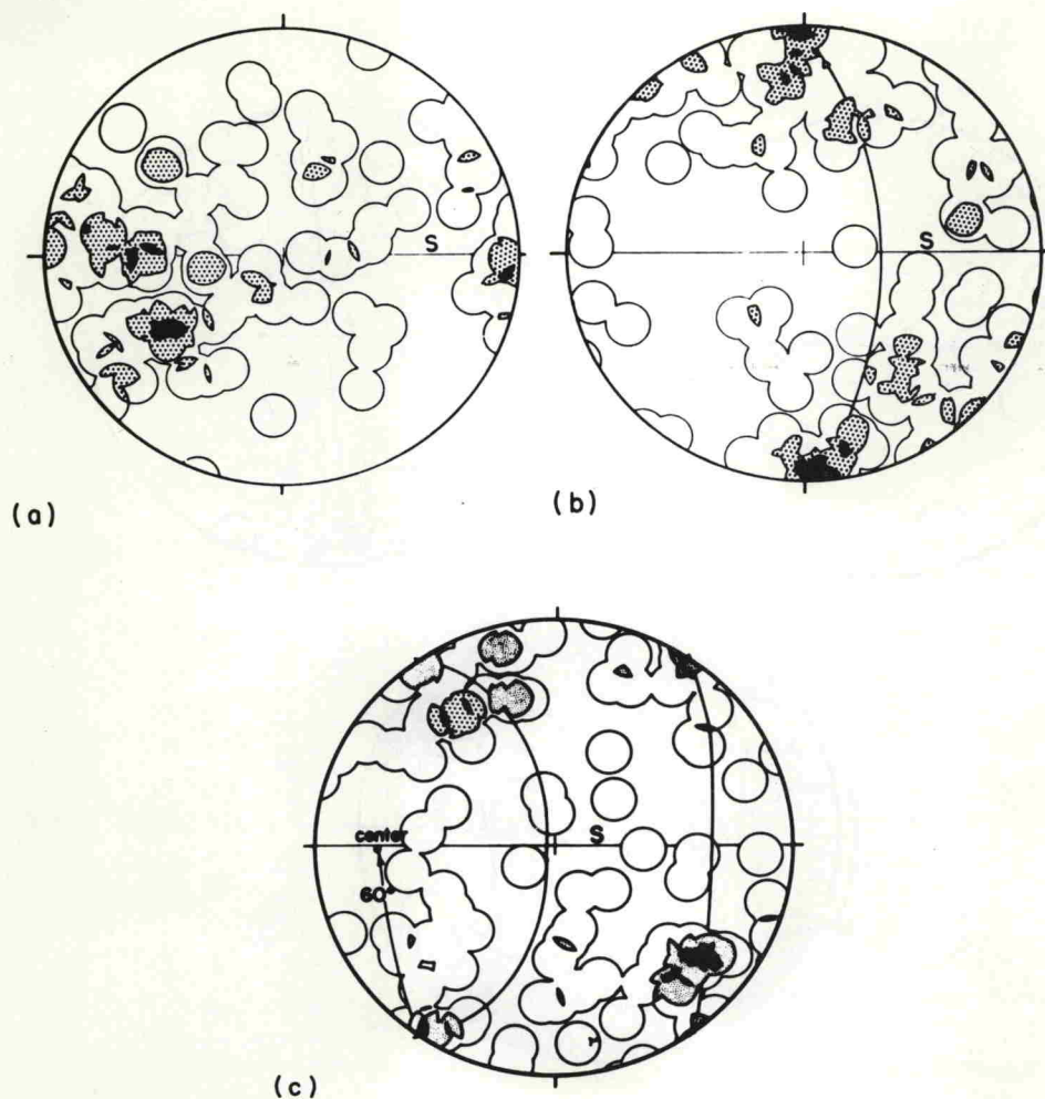
Fig. 45—Diagrams showing orientations of compression and extension axes (a and b) derived from calcite-cement twin lamellae and of quartz deformation lamellae (c) in Oriskany sandstone specimen E6 (from Hansen and Borg, Ref. 120, Figs. 8 and 9). Diagrams are oriented similar to those in Figs. 43 and 44. (a) 92 compression axes derived from the well-developed sets of e twin lamellae in 134 grains. Contours are at 1.1, 3.3, 5.5 per cent per 1 per cent area, 7.6 per cent maximum. (b) 92 extension axes. Contours are at 1.1, 3.3, and 5.5 per cent per 1 per cent area, 8.7 per cent maximum. Great circle defines the plane normal to the major concentration of compression axes. (c) Normals to 92 deformation lamellae in 210 grains. Contours are 1.1, 3.3, and 5.5 per cent per 1 per cent area, 5.9 per cent maximum. The center of the small circle is marked by a dot.
