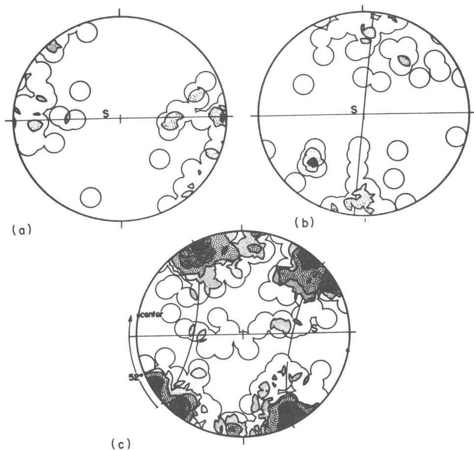
Fig. 44—Diagrams showing orientations of compression and extension axes (a and b) derived from calcite-cement twin lamellae and of quartz deformation lamellae (c) in Oriskany sandstone specimen E4 (from Hansen and Borg, Ref. 120, Figs. 6 and 7). Diagrams are oriented similar to those in Fig. 43. (a) 49 compression axes derived from the well-developed sets of e twin lamellae in 100 grains. Contours are at 2, 6, and 10 per cent per 1 per cent area. (b) 49 extension axes. Contours are at 2, 6, and 10 per cent per 1 per cent area. The great circle defines the plane normal to the major concentration of compression axes. (c) Normals to 220 deformation lamellae in 412 grains. Contours are at 0.5, 1.4, 2.3, 3.6, and 5.0 per cent per 1 per cent area, 7.3 per cent maximum. The center of the small circle defined by the normals to the lamellae is marked by a dot.
